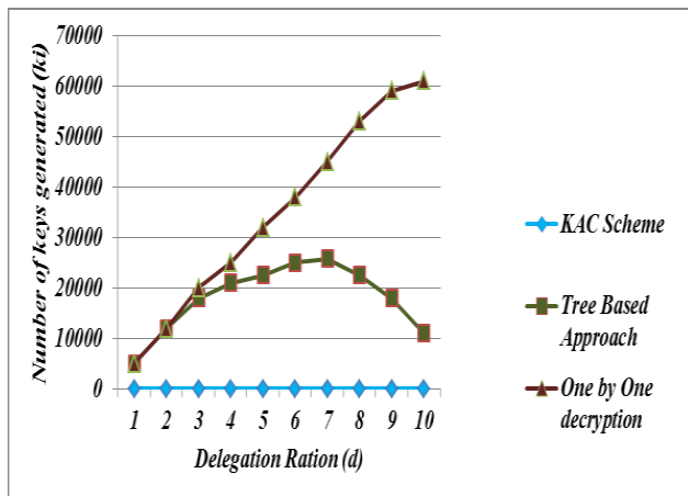
Figure.1 Comparison of KAC with the Existing Methods
